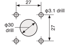
Mounting dimensions
