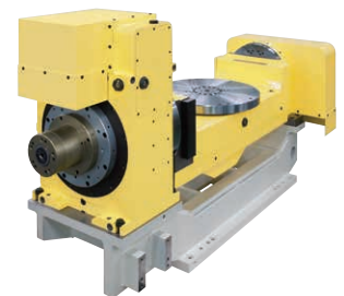
CNCB450T is used for the tilting axis table of 5AX-tilting rotary table.
