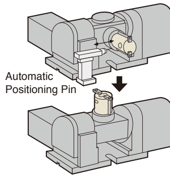
Bar removing after the machining of face mill cutter body
