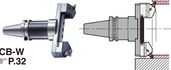
Stepped Boring
