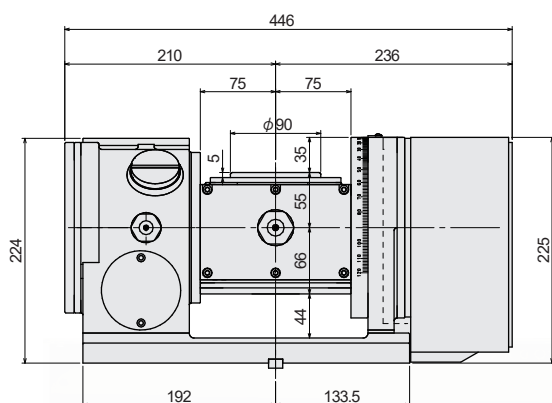
*Dimension : with AA21 controller
