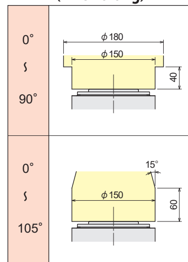
Interference area of work-piece (when tilting)
