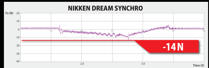
Tapping with the synchro tap holder with the fine floating (M6)
