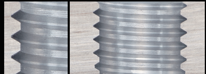
Tapping with NIKKEN DREAM SYNCHRO (M12)
