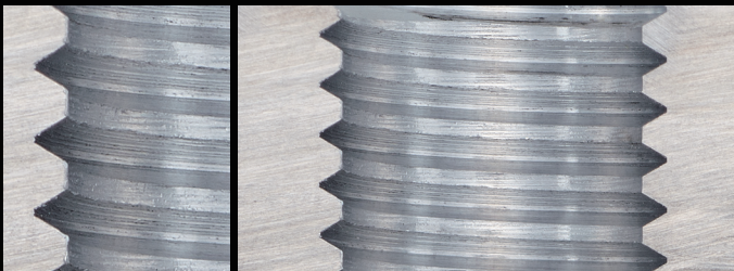
Tapping with the solid type holder (M12)
